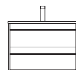
Lavabo encastre IBERIA 600/700/800/1000/1200
