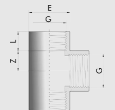
Material PVC-U
