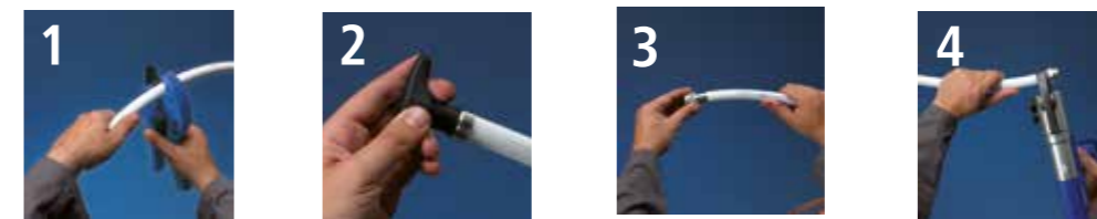
1 Cut the tube. 2 Calibration-beveled tube. 3 Assembling accessory. 4 Press.
